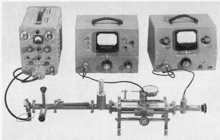
Figure 1. Set-up for waveguide measurements using new -hp- waveguide measuring instruments.
