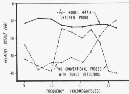
Figure 5. Typical response and efficiency characteristics of Model 444A untuned probe compared with conventional probes having tuned detectors.
