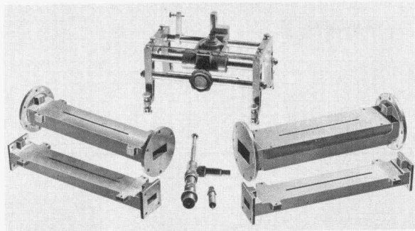
Figure 2. New set of waveguide slotted line equipment including 809B carriage assembly with four 810B slotted sections, and two broadband probes.
