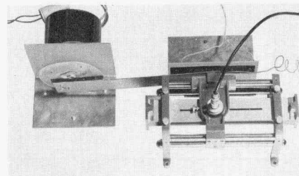
Figure 3. Breadboard set-up for motor drive for use with Model 809B carriage assembly.
