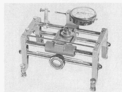
Figure 4. -hp- Model 809B carriage assembly with dial indicator.
