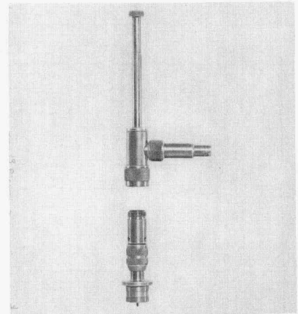
Figure 6. Model 440A detector mount (above) and 442A probe combine to make tuned slotted line probe. 440A will accommodate crystals, bolometers, or suitable fuses.
